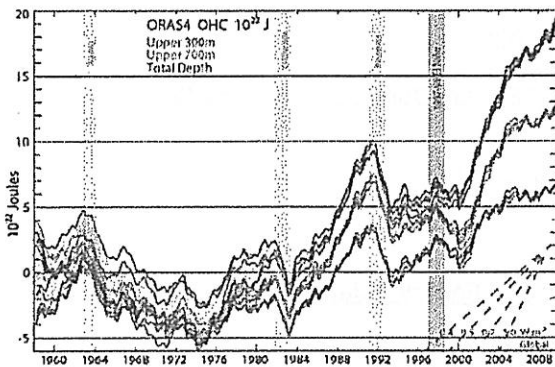
Source : Balmasida et al. Distinctive climate signals in reanalysis of global ocean heat content 1
