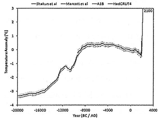
Source : Marcott et al. A Reconstruction of regional and global temperature for the past 11300 years
